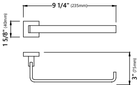
Model #: KEA-14425 Towel Bar Dimensions: 9 1/4" x 3" x 1 5/8"
