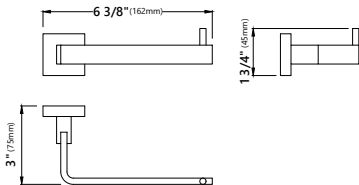
Model #: KEA-14429 Toilet Paper Holder Dimensions: 6 3/8" x 3" x 1 3/4"
