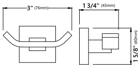
Model #: KEA-14401 Double Hook Dimensions: 3" x 1 3/4" x 1 5/8"
