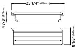
Model #: KEA-14442 Shelf with Towel Bar Dimensions: 25 \frac{1}{4}'' \times 8 \frac{1}{8}'' \times 4 \frac{7}{8}''
