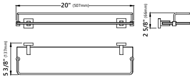
Model #: KEA-14445 Bathroom Shelf Dimensions: 20'' \times 5 \frac{3}{8}'' \times 2 \frac{5}{8}''
